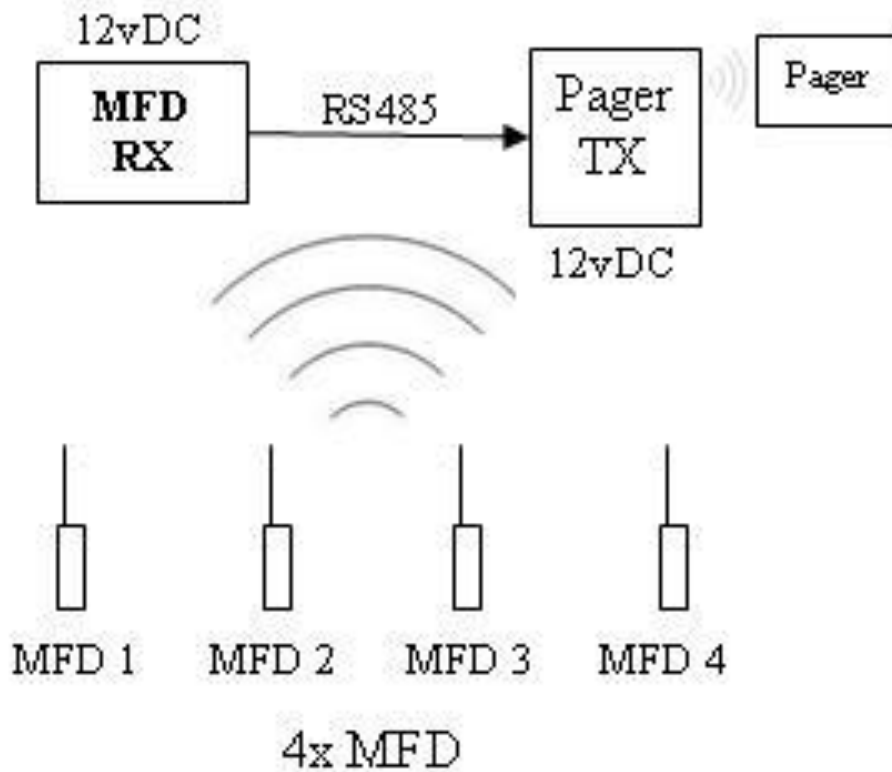
Figure 1. System schematic
